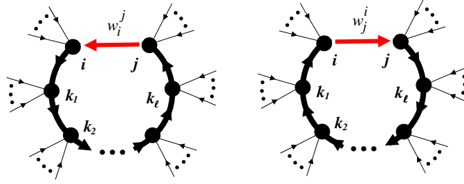
Figure 2. One term in [...] of equation (3), illustrating the emergence of nontrivial loops. Straight arrows (red online) represent the w factors; the rest (black online), the U 's. (This figure is in colour only in the electronic version)
